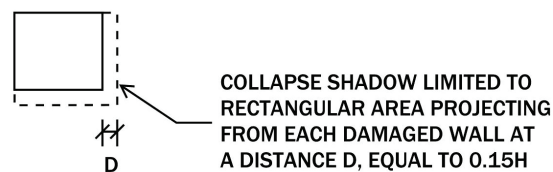
Figure 3-41 Plan sketch of recommended cordon shadow for rubble pile collapse mode.
