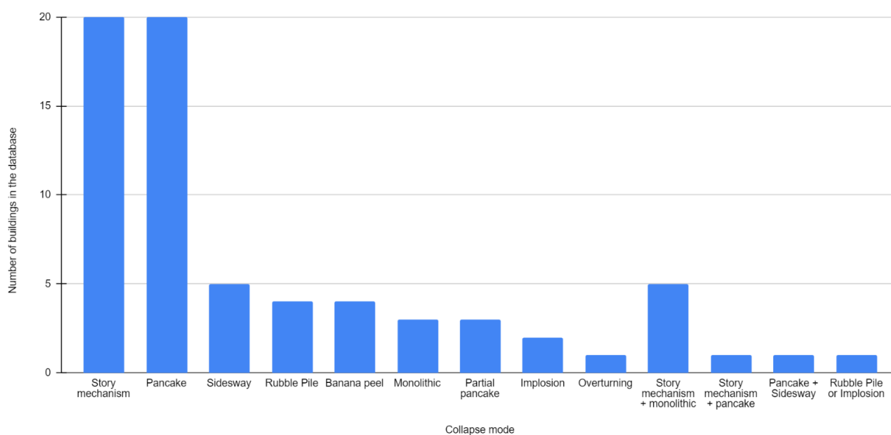
Figure A-6 Distribution of collapse modes for the buildings included in the database.
