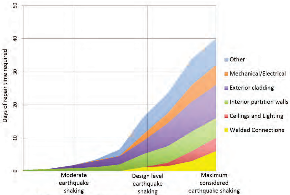
Median days of repair time required for different levels of shaking, broken out by components responsible.
