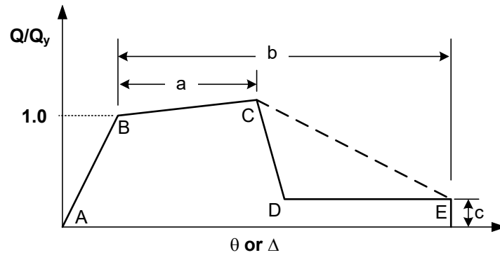
Figure 5-2 Generalized force-deformation relationship adapted from ASCE/SEI 41-13 (ASCE, 2014).
