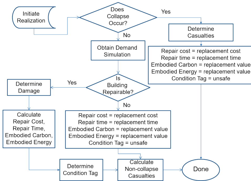
Figure 2-4 Flowchart for assessing a performance outcome in each realization.
