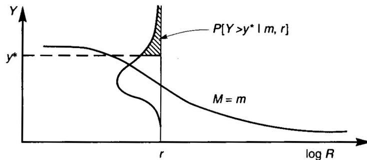
Figure B-6 Illustration of the conditional probability of exceeding a ground motion parameter (Kramer, 1996).
