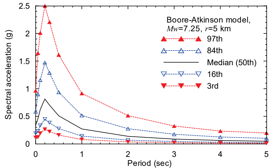
Figure 4-2 Response spectra with different probabilities of exceedance derived from a single ground-motion prediction equation for an earthquake scenario of M_w = 7.25 and r = 5 km.
