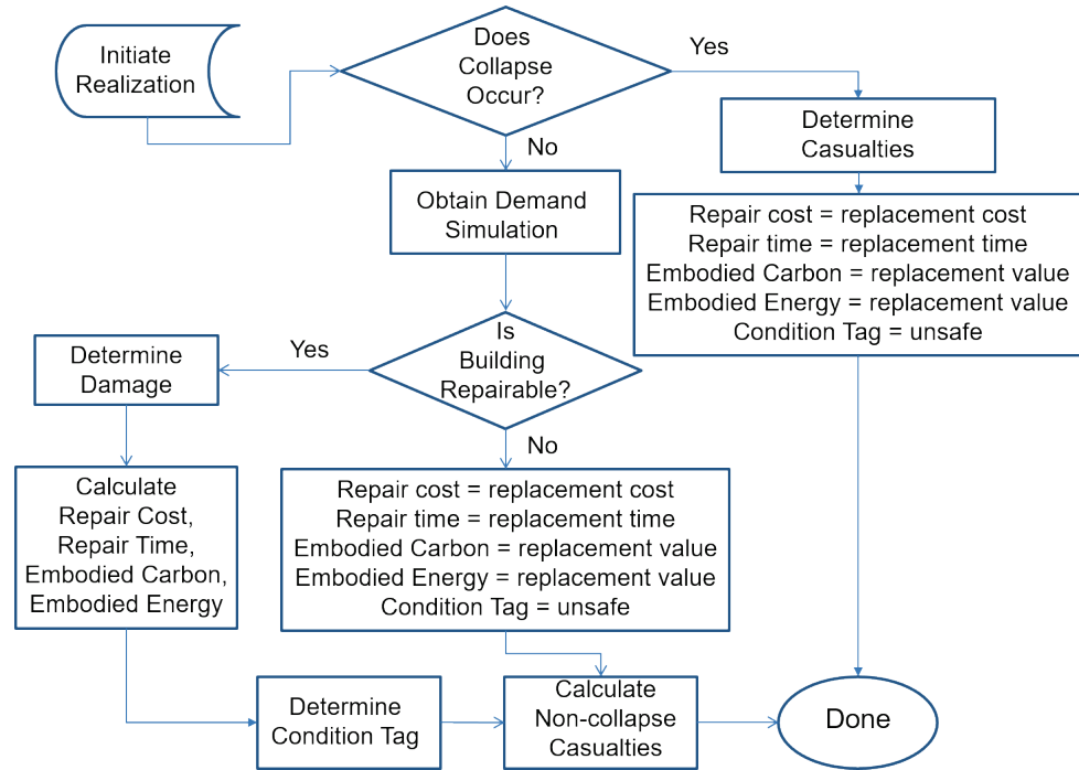
Figure 7-1 Flowchart for performance calculation in each realization.
