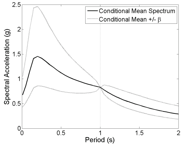
Figure B-11 Conditional Spectrum for S_a(1s) with 2% probability of exceedance in 50 years for a rock site in San Francisco.
