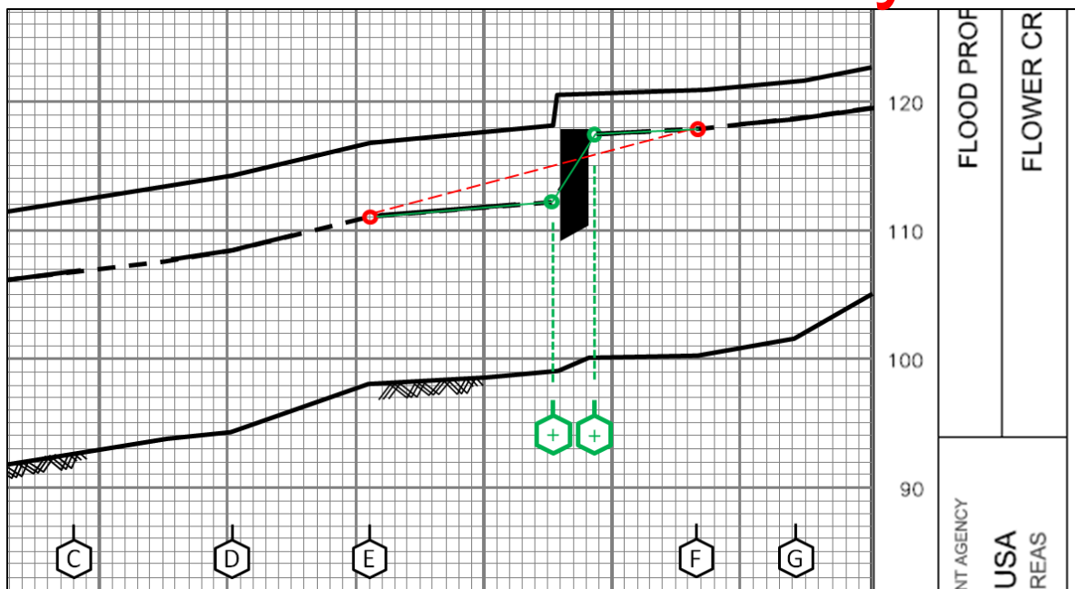
Figure 7: All Modeled Cross Sections are Necessary for Accurate Grid Representation
