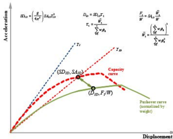
FIGURE C18.7-2 Pushover and Capacity Curves
