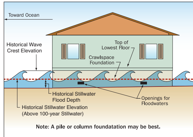
Figure 8. Recommended construction in Zone B, Zone C, and Zone X.
