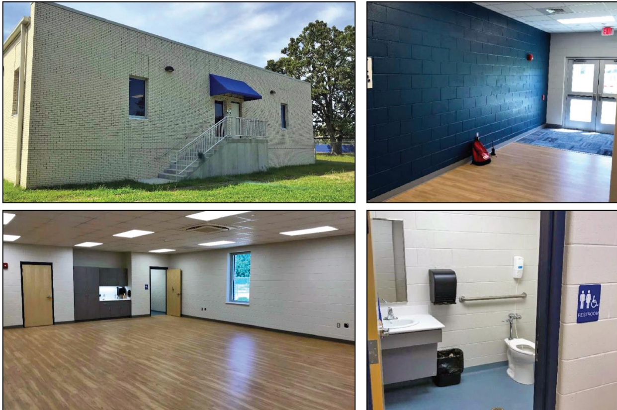
Figure A3-1: The addition to this school was designed to serve as a multi-use safe room; it is also used as a cafeteria, gym, and large-group gathering space (Climax Springs, Missouri)
